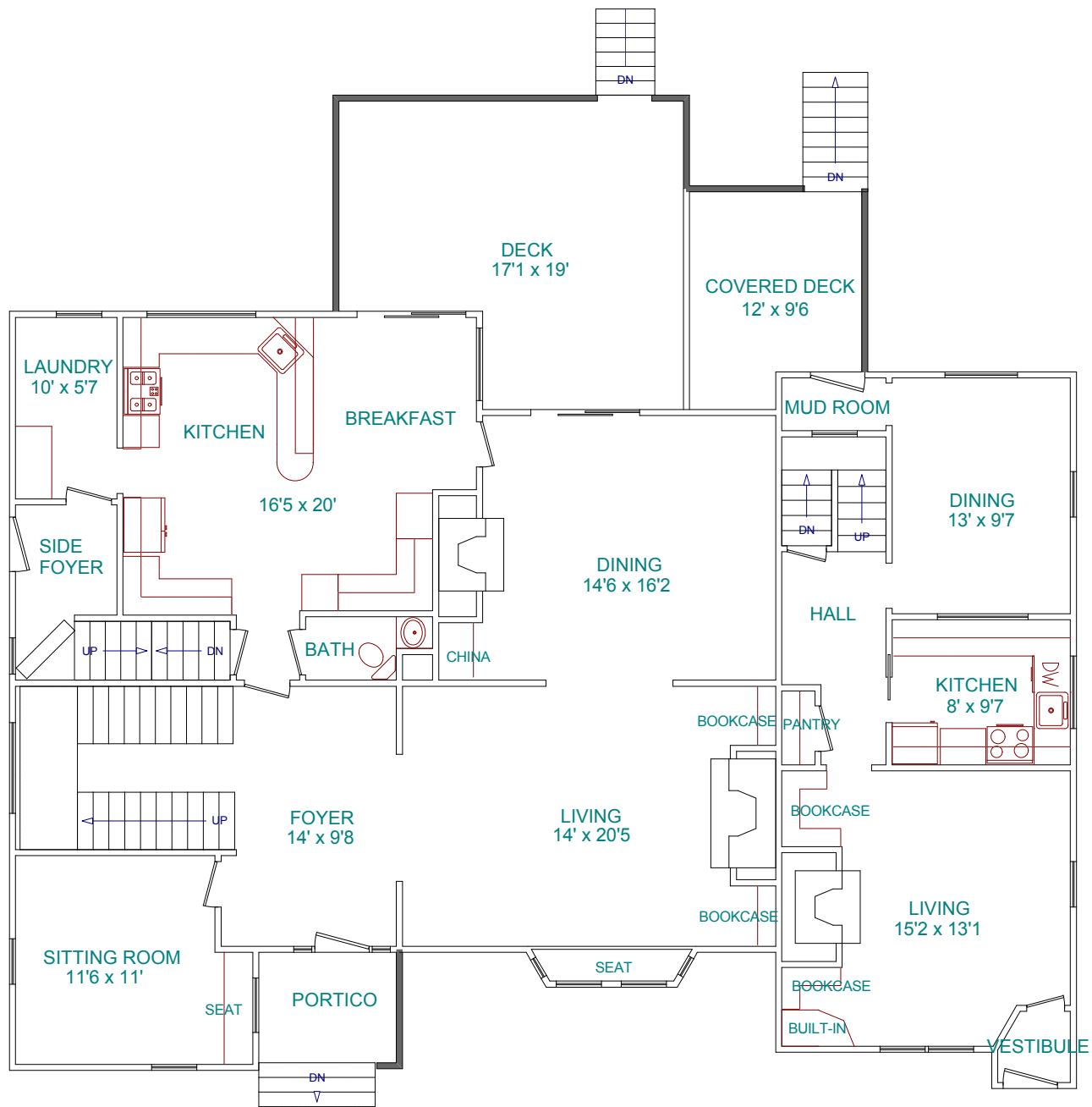
First Floor Main House
